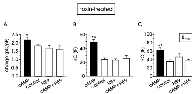
FIGURE 8 Potentiation of exocytosis in toxin-treated cells is mediated by PKA (A) Mean quantity of charge during 100-ms depolarization at +10 mV with the solutions indicated. In all cases, cells were previously incubated with toxins. Quantity of charge with pCPT-cAMP significantly differed from control, H89-treated cells, and those incubated with H89 + pCPT-cAMP ( P < 0.05 ) (B) Mean ΔC increases in different experimental conditions. Statistical significance was P < 0.01 . (C) The maximum size of the RRP estimated with the dual-pulse protocol. The secretory response with cAMP is statistically different from that of all the other groups ( P < 0.01 ).
