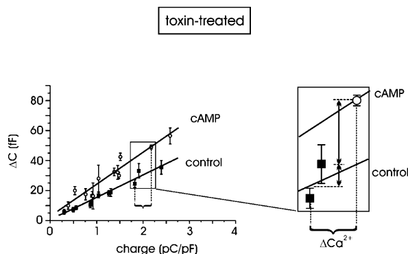
FIGURE 4 Calcium dependence of exocytosis in toxin-treated cells. Capacitance increments plotted versus the quantity of charge: each abscissa point is the mean charge value for the corresponding pulse length (from 10 to 150 ms). Standard errors on abscissas are omitted for clarity. In the range examined, \Delta C data are positively correlated with the quantity of charge; linear regression for control and pCPT-cAMP-treated cells gave 15.1 \pm 0.9 vs. 21.4 \pm 1.7 fF/(pC/pF), respectively. Inset: see text for details.
