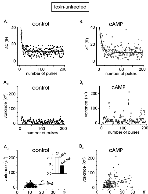
FIGURE 7 cAMP increases the single quantal size. Nonstationary statistical analysis of the secretory responses evoked by 20-ms depolarizations at +10 mV repeated at 0.3-Hz frequency for control (A) and pCPT-cAMP-treated (B) cells. (A 1 , B 1 ) ΔC values measured in response to consecutive depolarizations for two representative cells. (A 2 , B 2 ) Sample variances versus time calculated from panels A 1 and B 1 . (A 3 , B 3 ) Plot of variances versus the corresponding means. Linear regression (solid line) had a slope of 0.9 fF (control) and 2.3 fF (cAMP). Dotted lines represent the confidence limits of the fit (95%). Inset: mean quantal size for control ( n = 9 ) and cAMP-treated cell ( n = 10 ), P < 0.01 .
